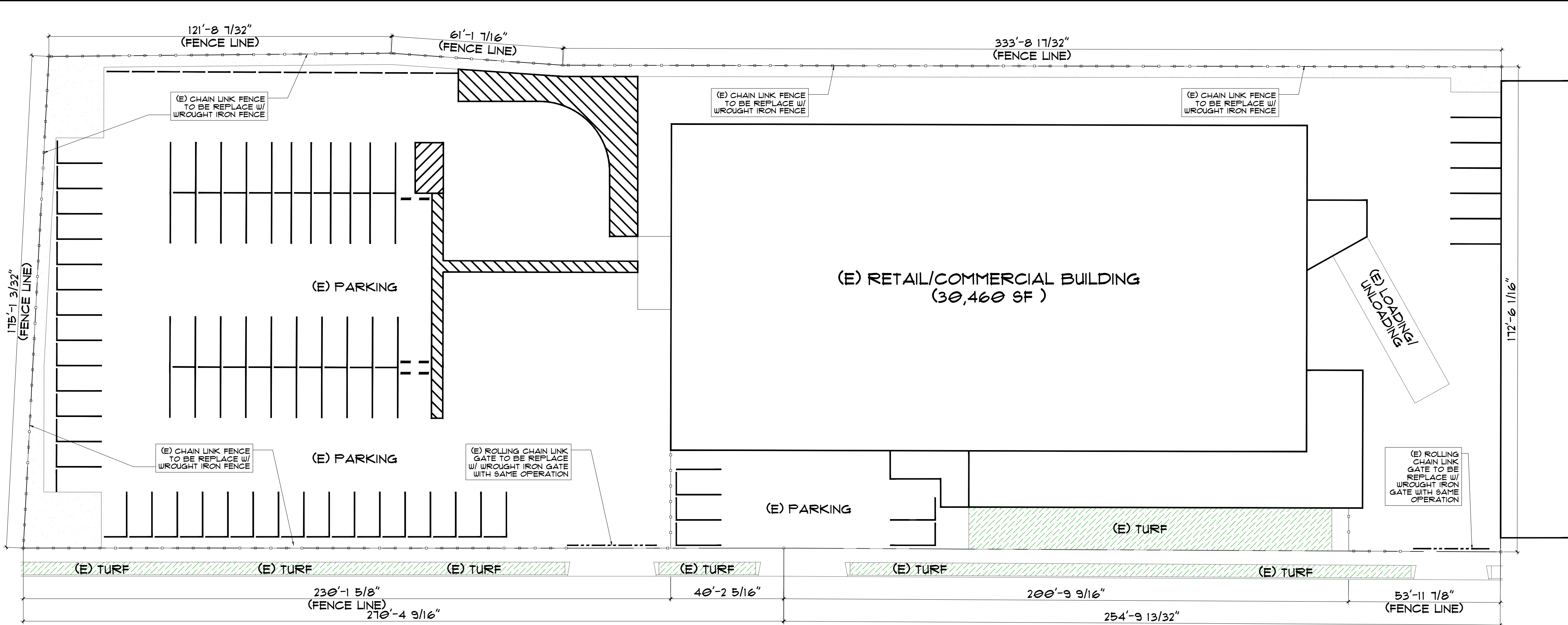
1 (E) PLOT PLAN SCALE: 3/64"=1'-0" NORTH
