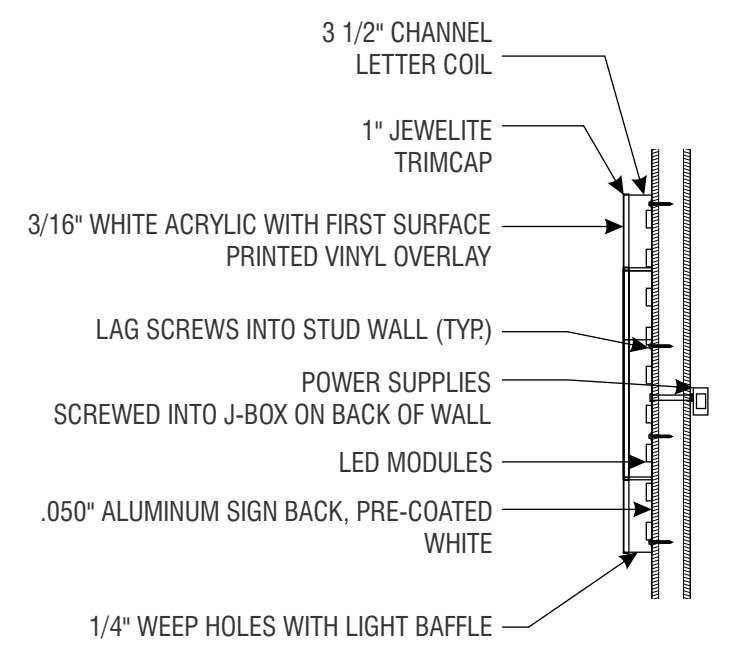
SECTION VIEW SCALE: 1/2" = 1'-0"
