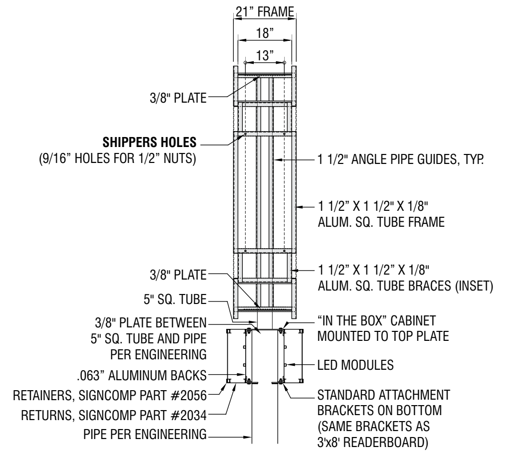
SECTION VIEW SCALE: 3/8"=1'-0"
