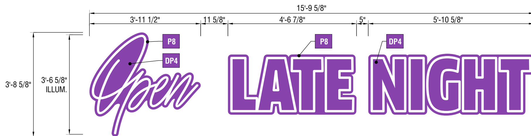
FRONT VIEW 58.76 SQ. FT. SCALE: 1/2" = 1'-0"
