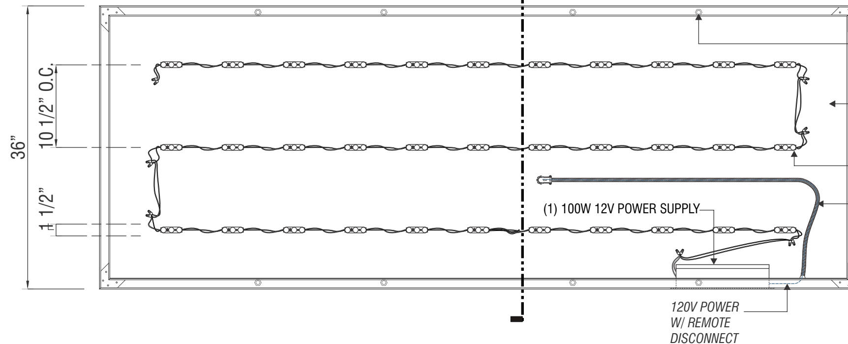
FRONT VIEW - CABINET ASSEMBLY, NO FACE
