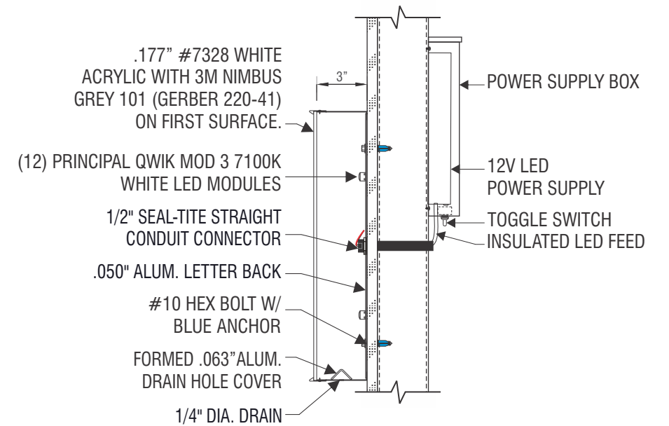
SECTION VIEW
