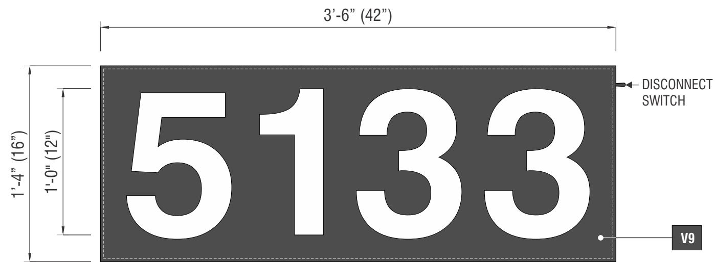
FRONT VIEW
