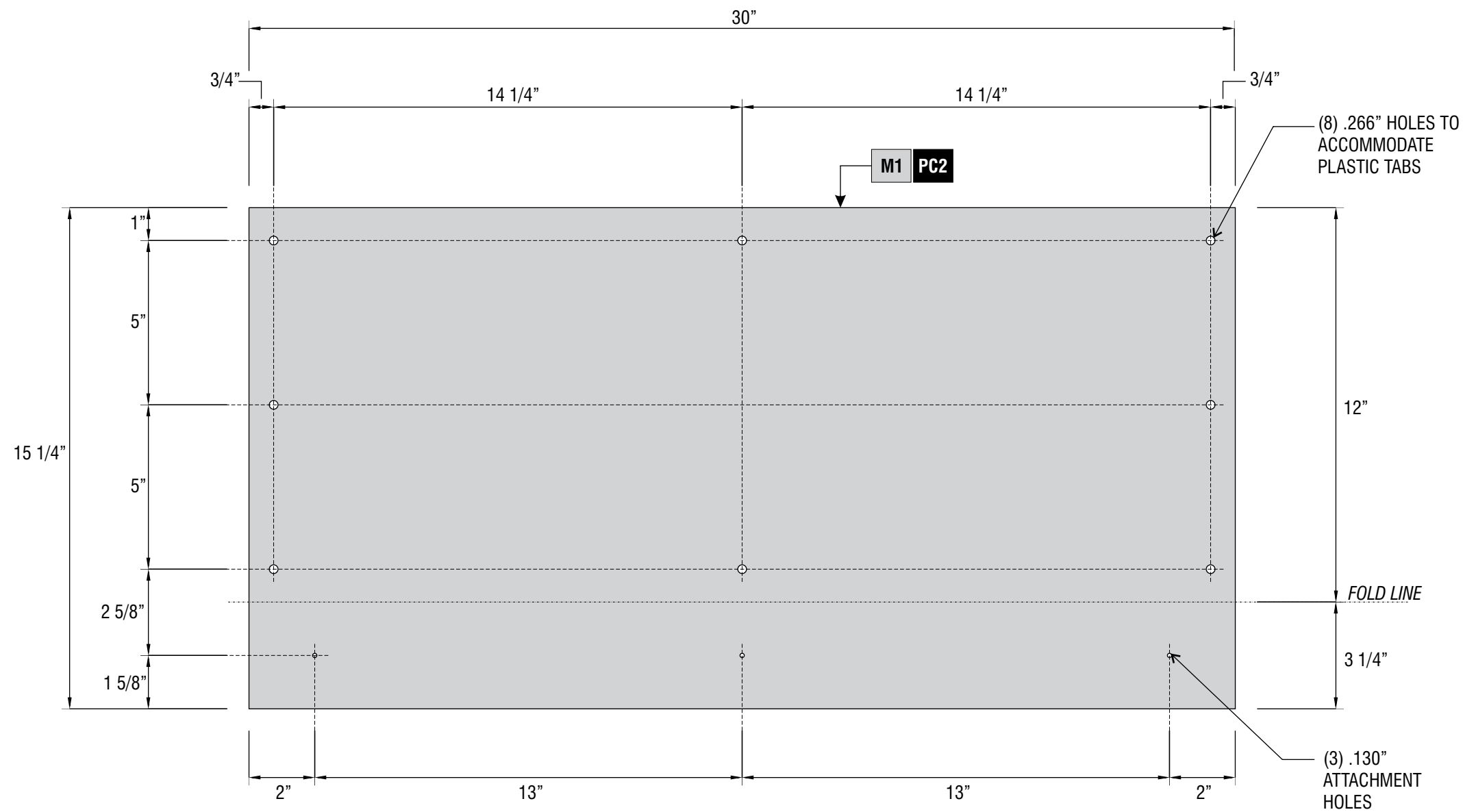
FRONT VIEW (BEFORE FOLD)
